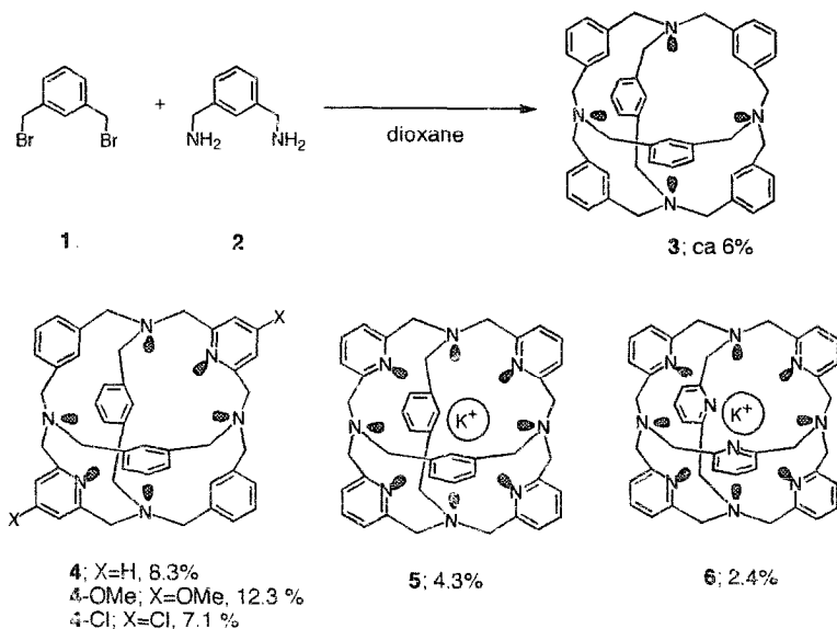
Scheme 1. Synthetic scheme of hexametyxylylenetetramine 3 and its pyridine analogs 4–6 .
