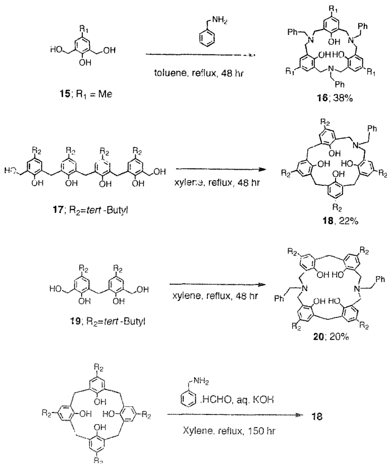
Scheme 4. Synthesis of azacalix[ n ]arenes 16 , 18 and 20 .
