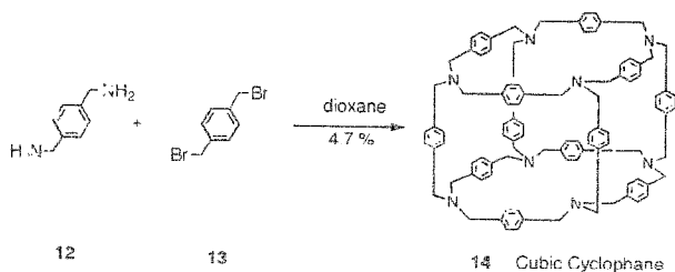
Scheme 3. Direct synthesis of cubic cyclophane 14 .
