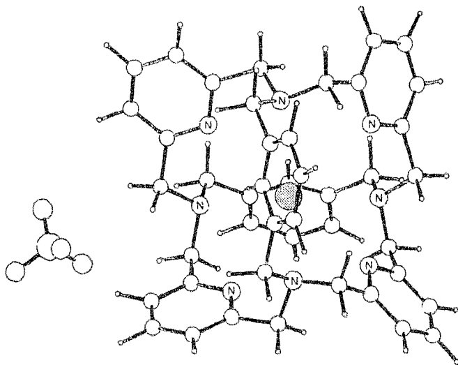
Fig. 1. X-ray structure of \text{K}^+ \cdot 5\text{ClO}_4^- \cdot \text{CHCl}_3 ; chloroform molecule is omitted. \odot shows \text{K}^+ ion.
