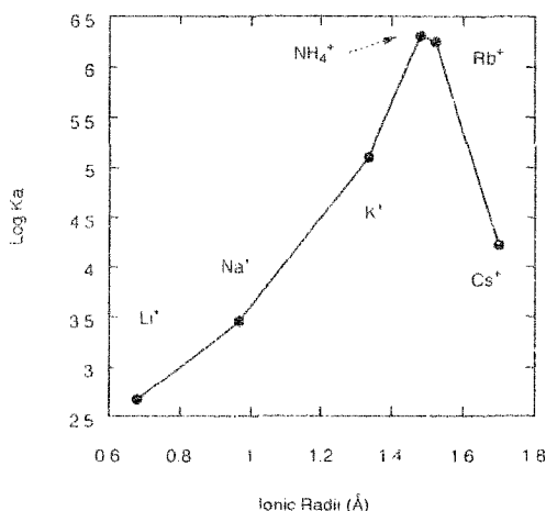
Fig. 2. Plots of association constants of M^+ \subset 5 vs. ionic radii of M^+ .
