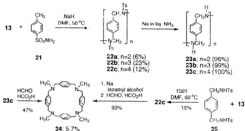
Scheme 5. Synthesis of (Ts) 4 N n [3 n ]azacyclophanes by one-step and two-step p -toluenesulfonamide method.
