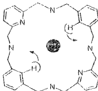
Fig. 4. Flipping of aromatic inner protons of M^+ @ 5 depends on the size of guest cations, M^+ . Pyridine units in front and back are oriented.
